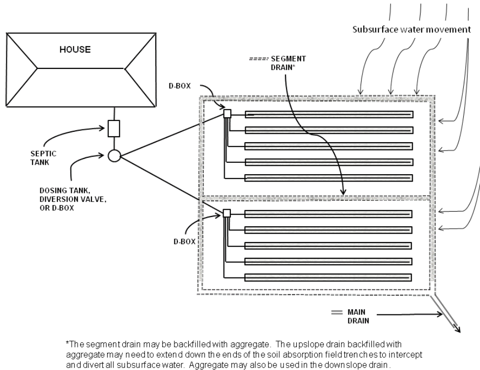
Figure 4: Subsurface Perimeter Drain with a Segment Drain on a Sloping Site
