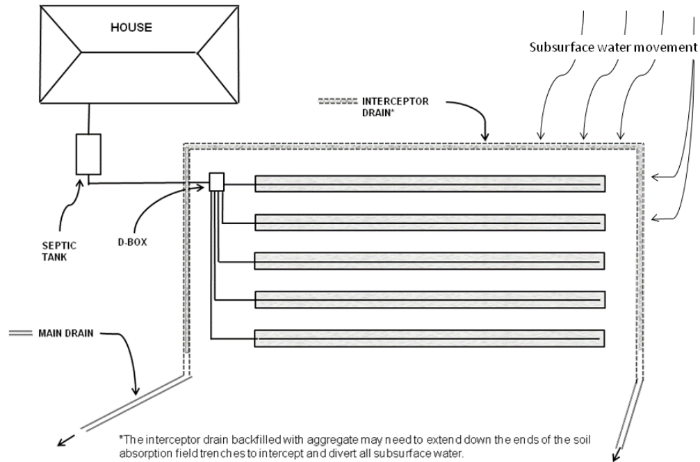
Figure 4: Subsurface Perimeter Drain with a Segment Drain on a Sloping Site
