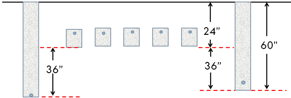
Figure 6: Perimeter Drain Depth for a SAF on a Sloping Site
